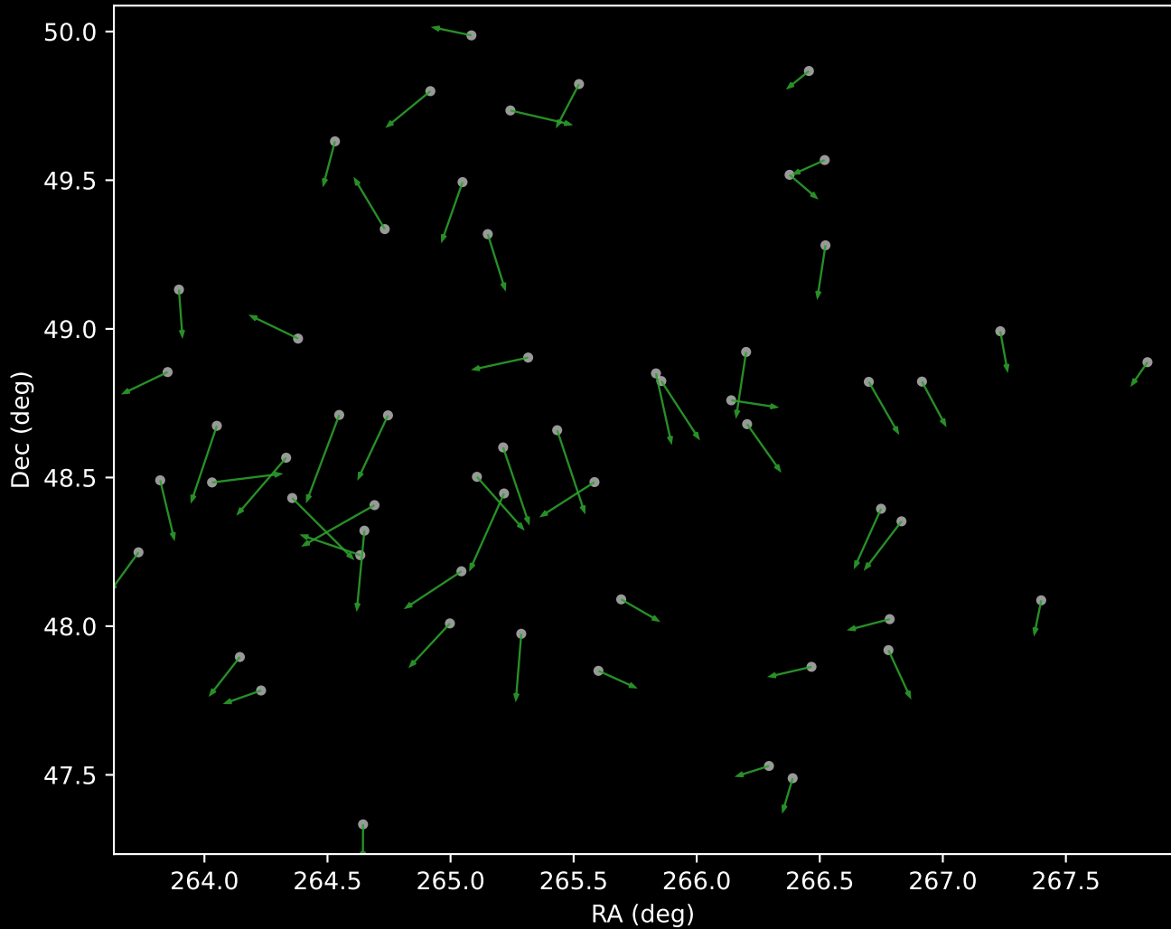
APOGEE DR17 Cluster 4 Proper Motion Vectors (n=57)
