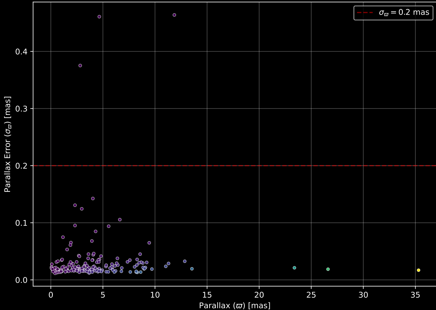
APOGEE DR17 Field: [160+60] Parallax Quality (n= 187)
