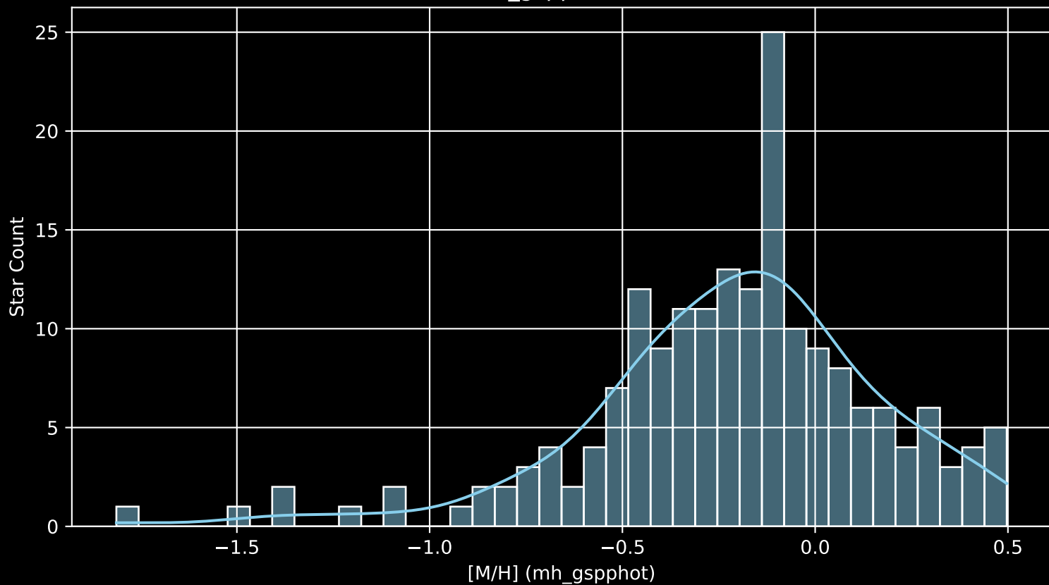
APOGEE DR17 Field: [160+60 [M/H] (mh_gspphot) (n= 186)
