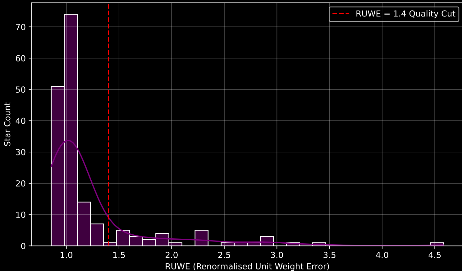
GAPOGEE DR17 Field [160+60] RUWE Distribution (n= 176)
