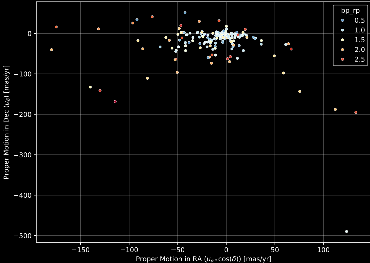
APOGEE DR17 Field: [160+60] Proper Motion Diagram (n= 187)
