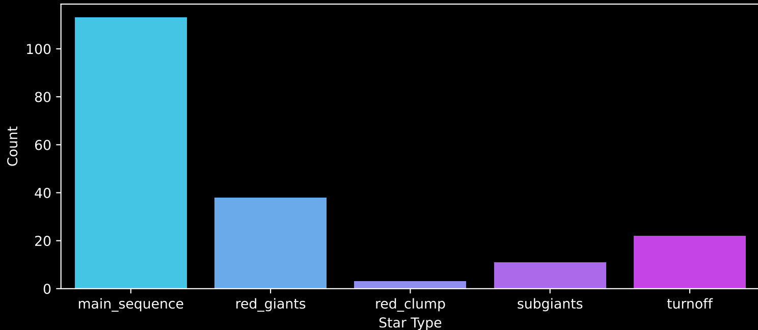
APOGEE DR17 Field: [160+60] Count plot of Star Type
