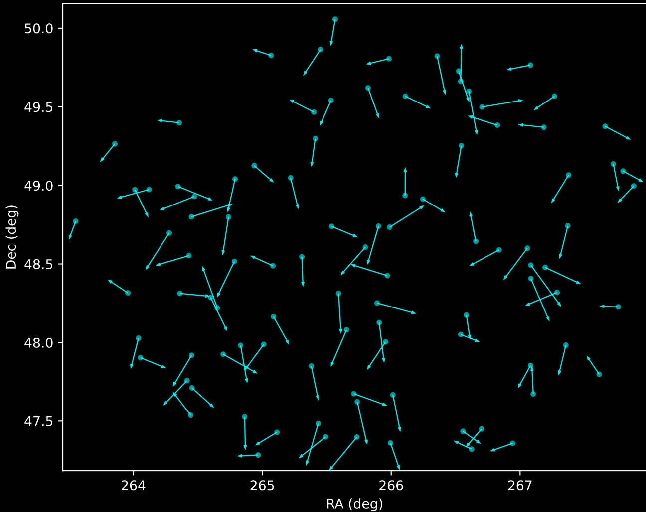
APOGEE DR17 Noise Stream Proper Motion Vectors (n=97)
